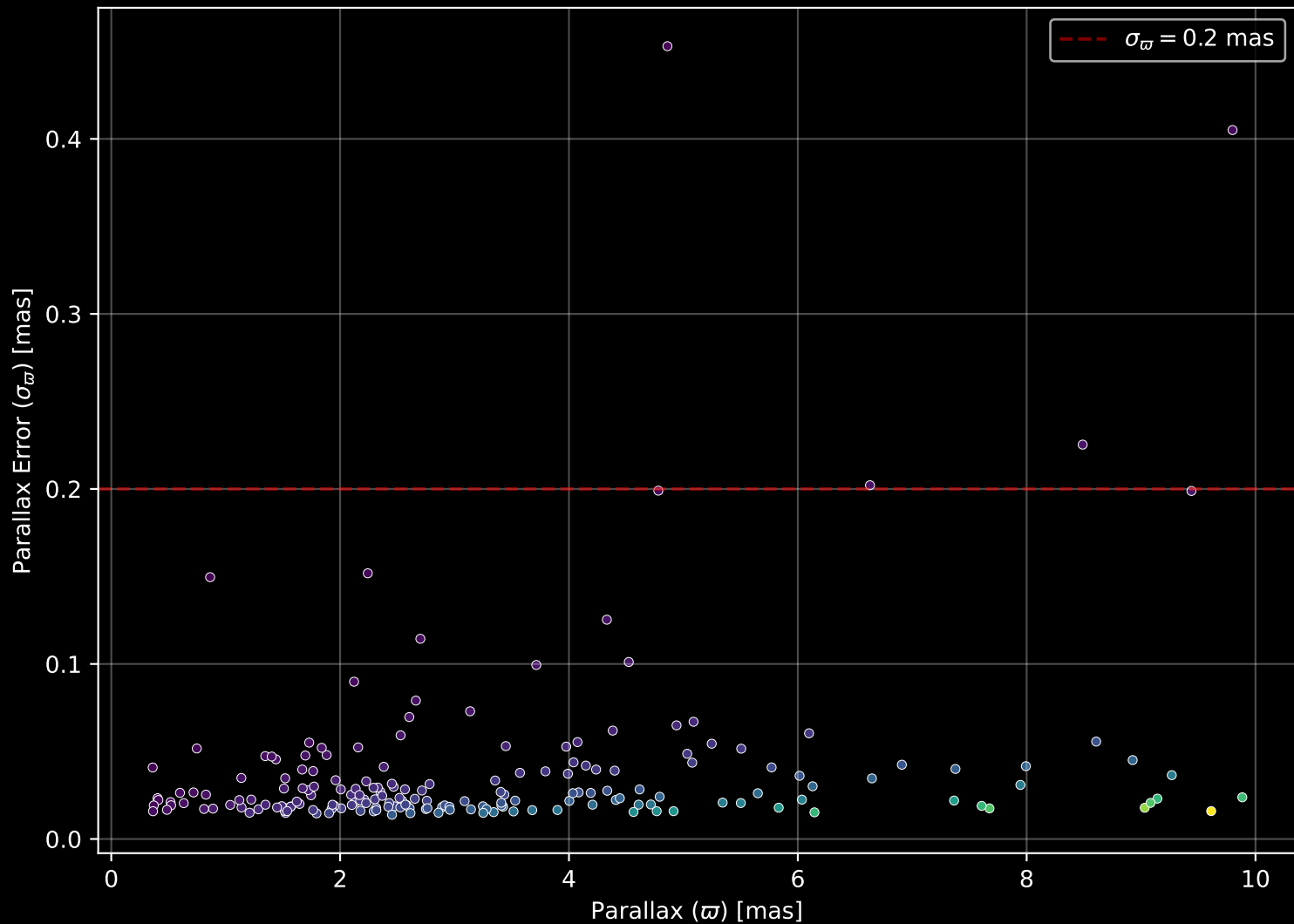
APOGEE DR17 Field: [K2_C8_129-57] Parallax Quality (n= 193)
