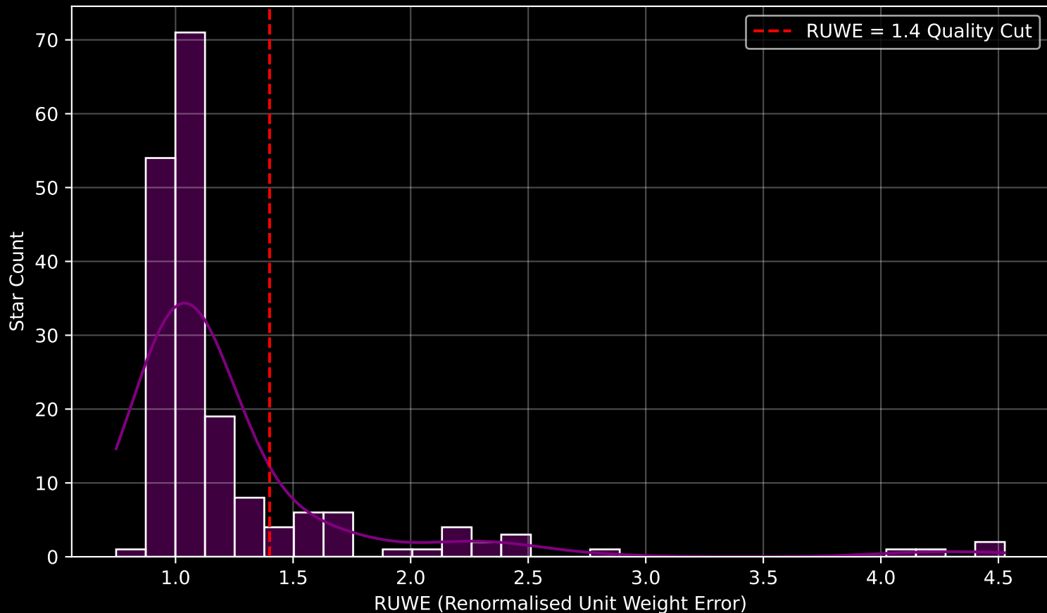
GAPOGEE DR17 Field [K2_C8_129-57] RUWE Distribution (n= 185)
