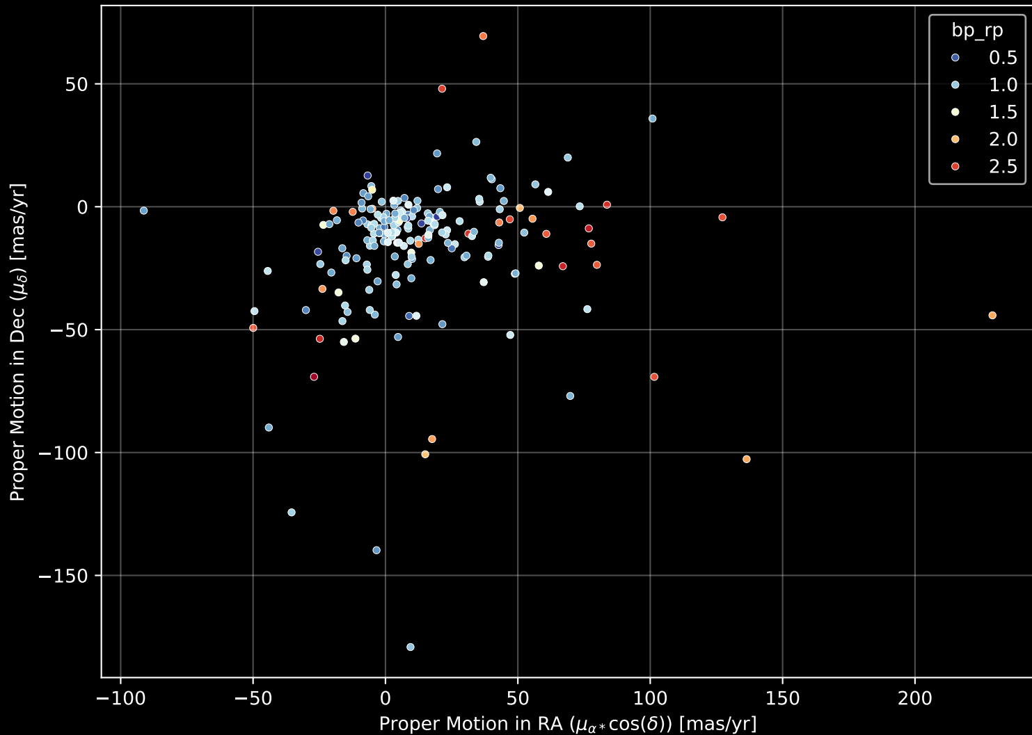
APOGEE DR17 Field: [K2_C8_129-57] Proper Motion Diagram (n= 193)
