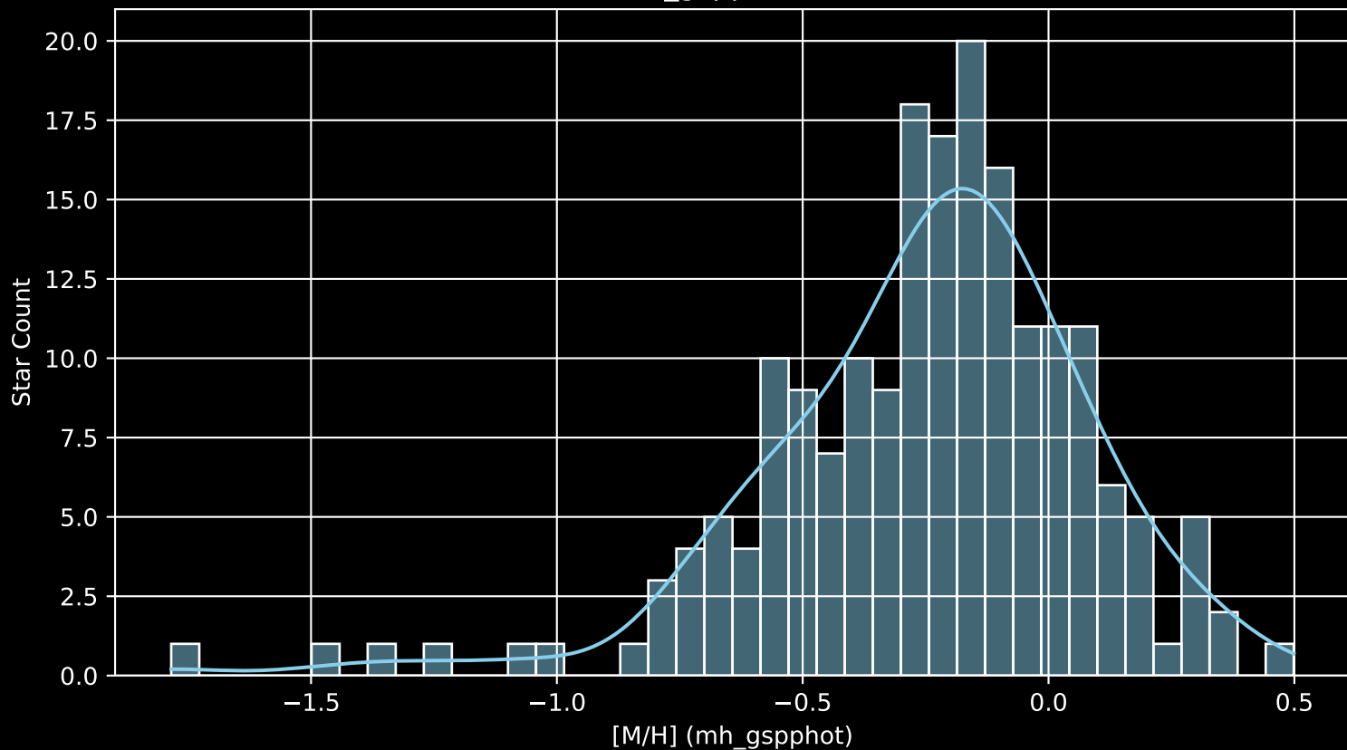
APOGEE DR17 Field: [K2_C8_129-57 [M/H] (mh_gspphot) (n= 192)
