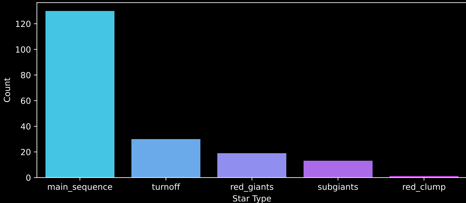
APOGEE DR17 Field: [K2_C8_129-57] Count plot of Star Type
