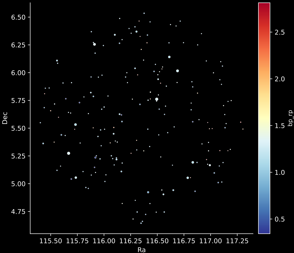
APOGEE DR17 Field: [K2_C8_129-57] Stars: 193
