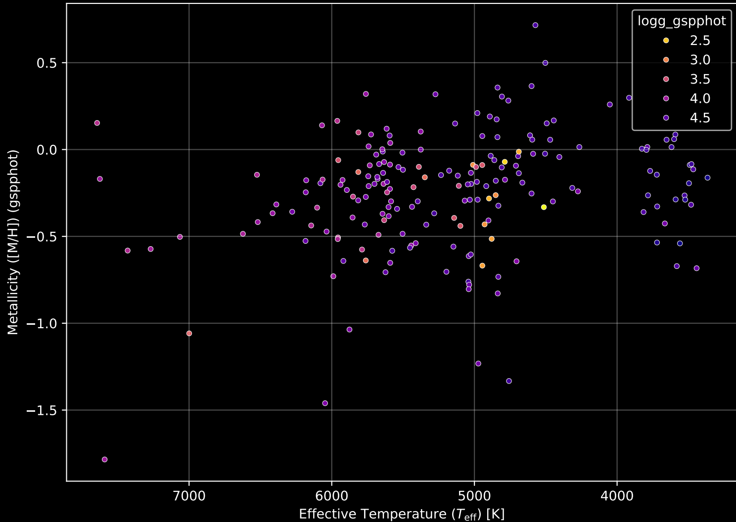
APOGEE DR17 Field: [K2_C8_129-57] Stellar Population Parameters (n= 193)
